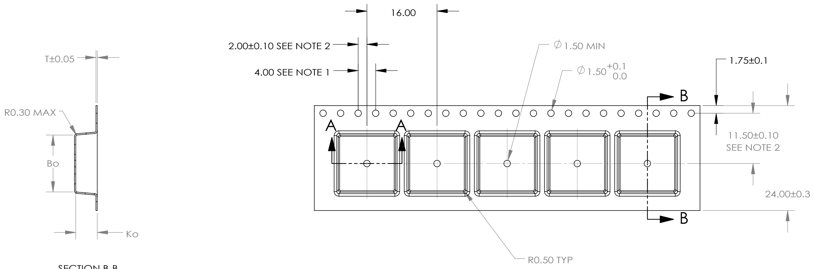
SECTION B-B
